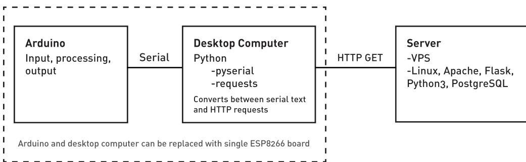
Fig. 3. Setup for prototyping.
